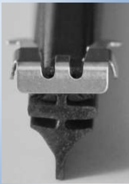
Fig. 1 Standard-rubber with metalclip
